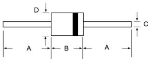
DO-201
