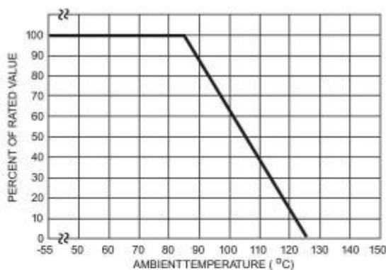
Figure 1A - Power Derating for Epoxy Coated
