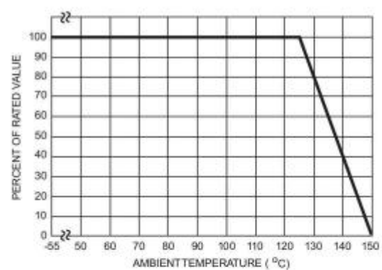
Figure 1B - Power Derating for Pholenic Coated
